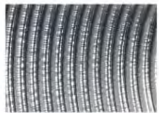
N12 R a 50 µm – AARH / CLA 2000 R z 185 µm
